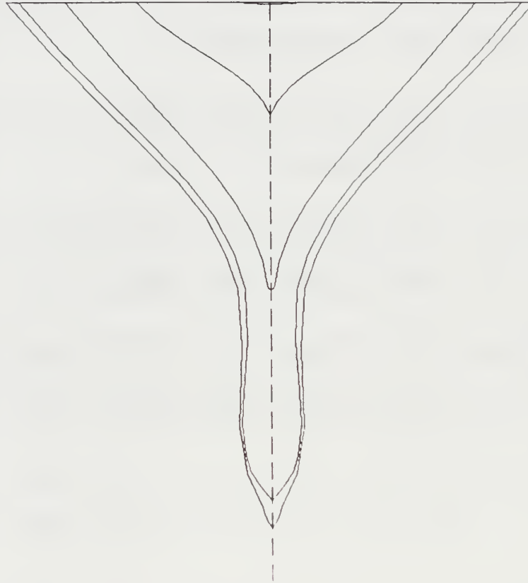
FOREPEAK.C Body Plan (1 component) Scale = 1:100
